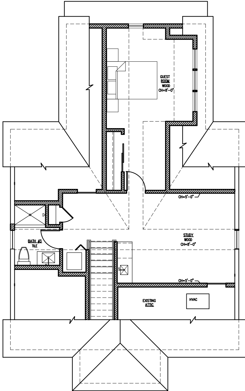
1 ATTIC FLOOR PLAN SCALE: 1/8" = 1'-0"
